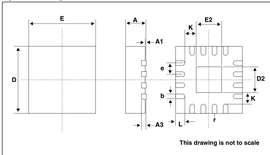
Figure 27. Package dimensions
